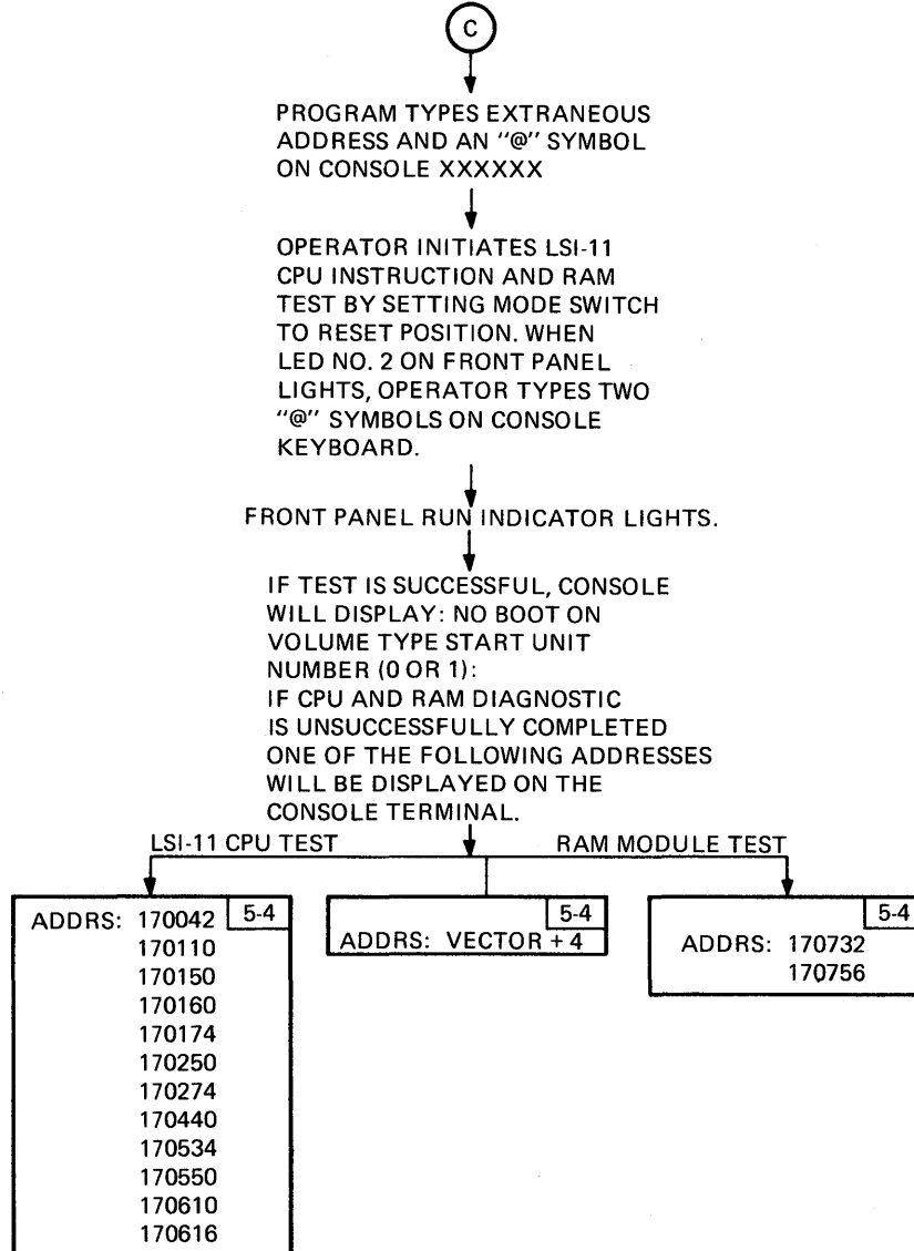
FIG. 5-2 (SHEET 2)
