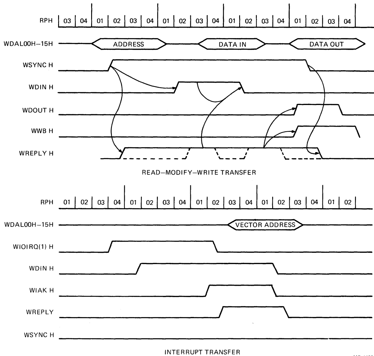
Figure 4-10 LSI-11 Microprocessor, I/O Transfer Timing (Sheet 2 of 2)
