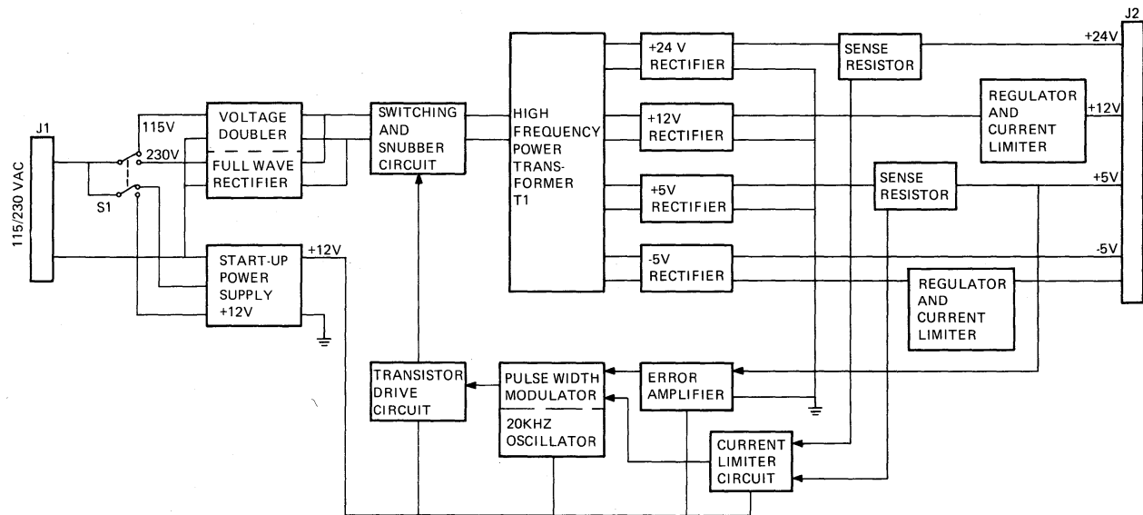
Figure 4-47 H7833 Power Supply, Simplified Block Diagram
