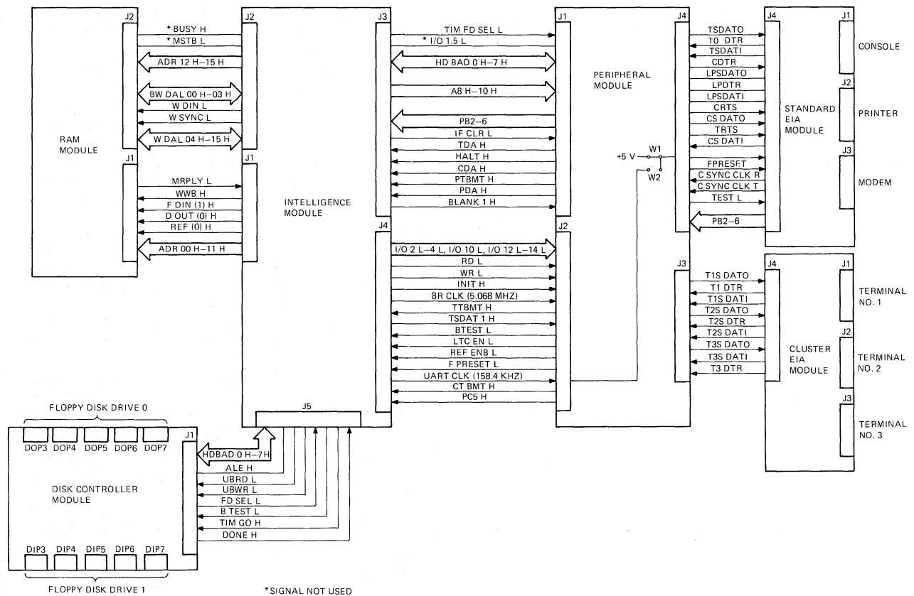
Figure 4-3 PDT-11/150 Internal Signal Distribution
