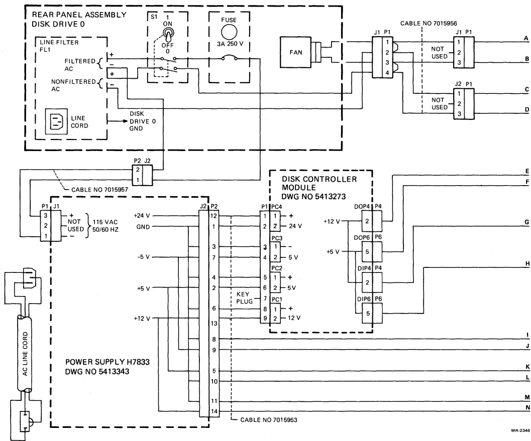
Figure 5-5 AC/DC Power Distribution, 60 Hz Units (Sheet 1 of 2)
