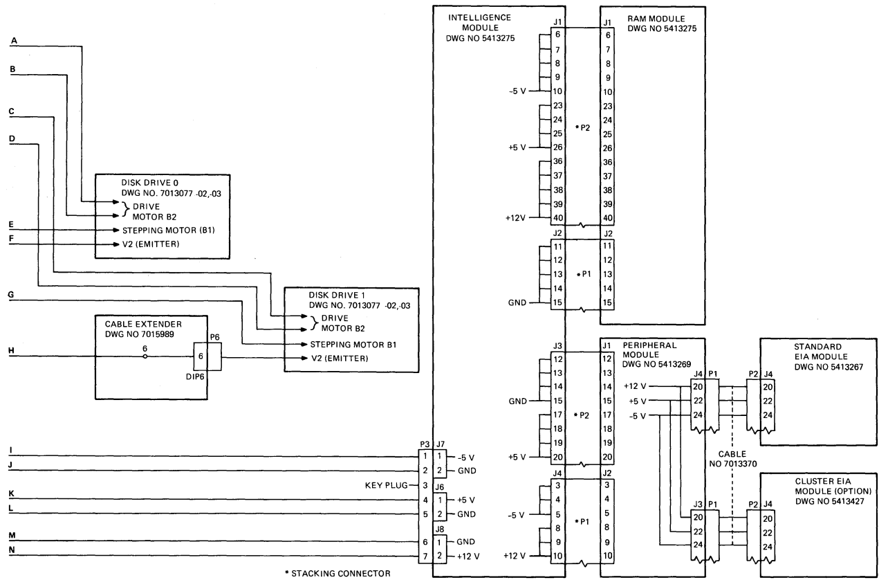
Figure 5-5 AC/DC Power Distribution, 60 Hz Units (Sheet 2 of 2)
