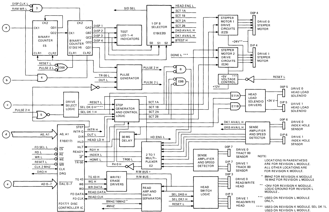
Figure 4-30 Disk Controller Module, Simplified Function Diagram (Sheet 2 of 2)
