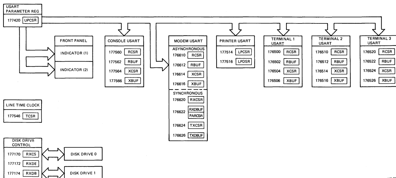
Figure 6-2 PDT-11/150 Device Register Address Assignments
