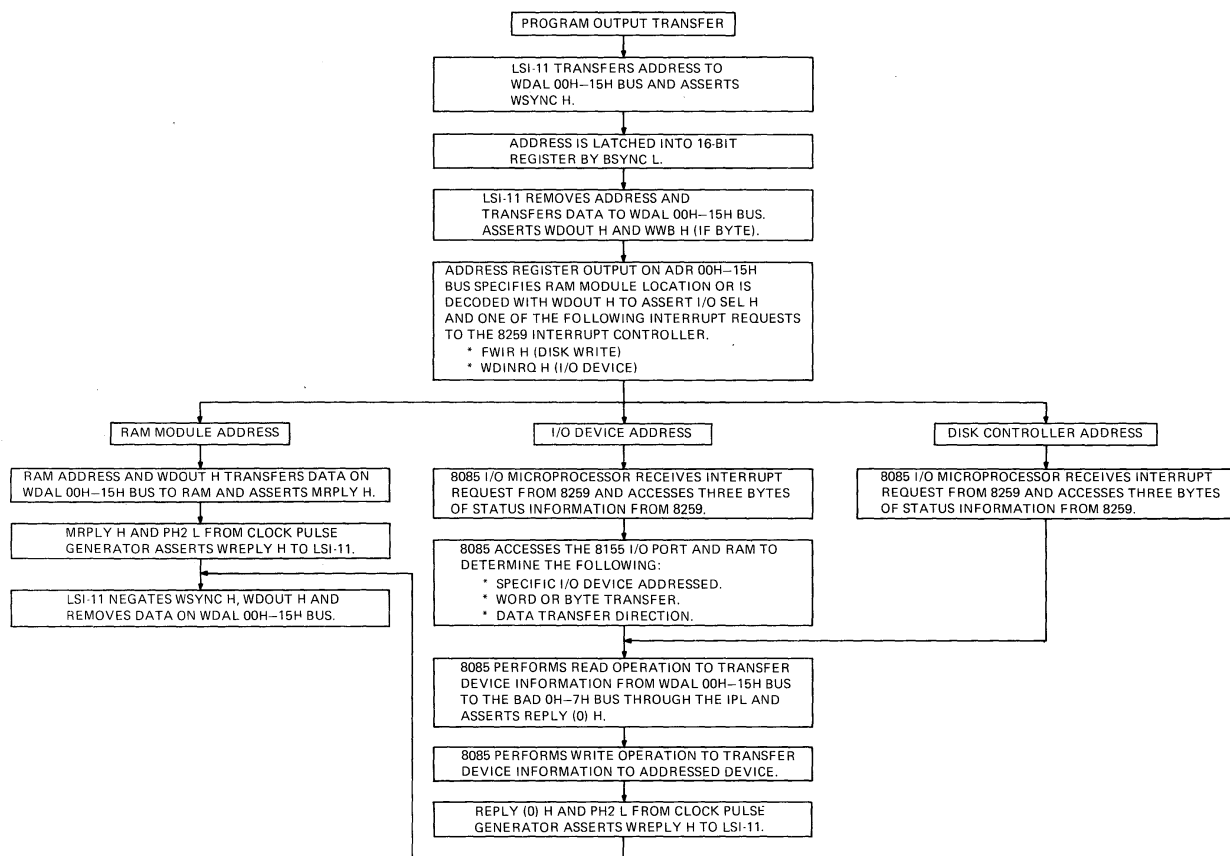
Figure 4-11 Output Transfer Events
