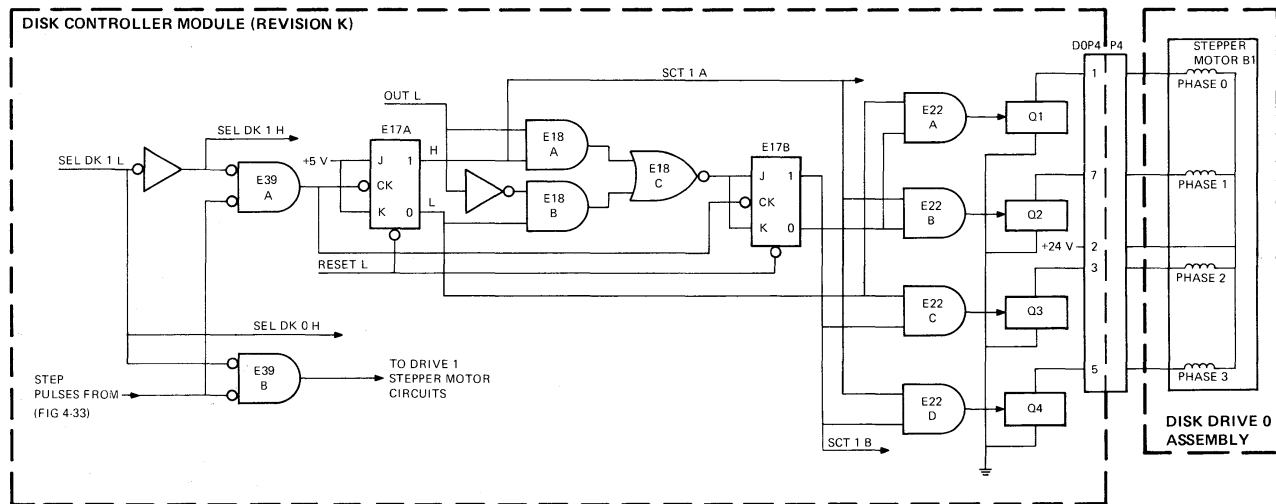
Figure 4-35 Stepper Motor Control and Drive Logic (Revision K), Simplified Diagram
