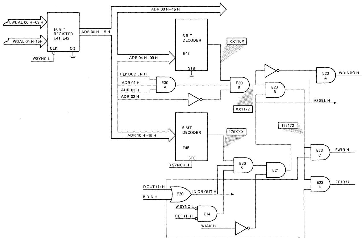
Figure 4-14 LSI-11 I/O Device Address Decoding Logic, Simplified Diagram
