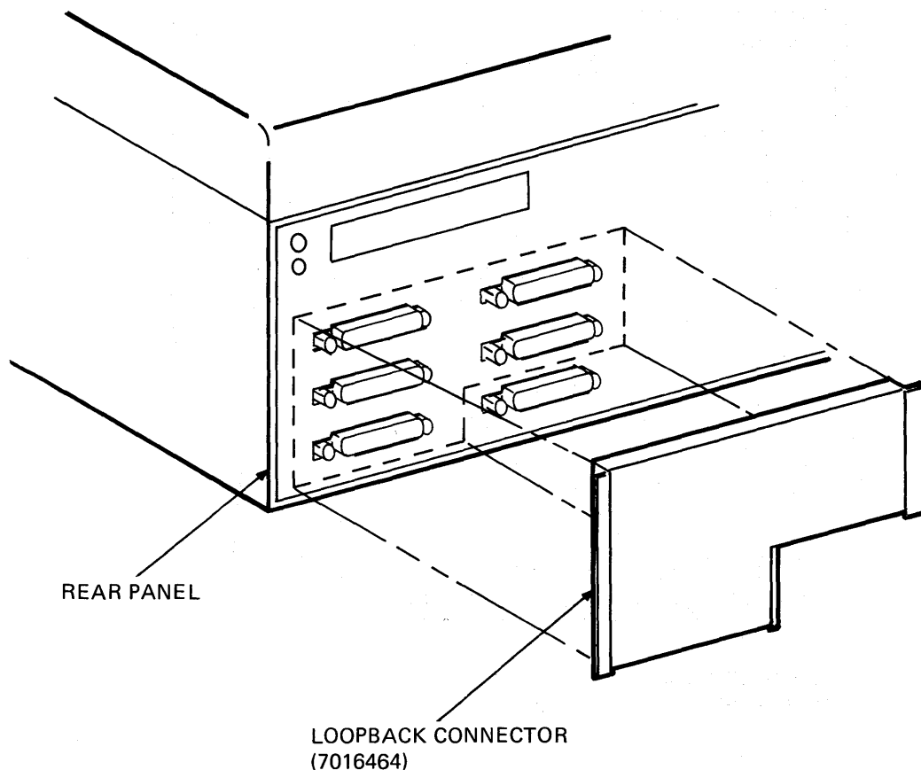
Figure 3-3 Loopback Connector Installation
