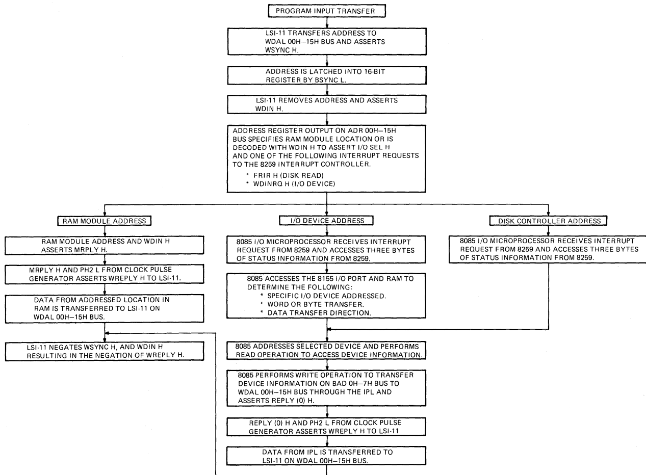
Figure 4-12 Input Transfer Events
