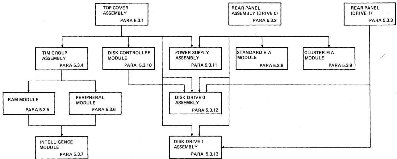
Figure 5-19 PDT-11/150 Removal and Replacement Reference Chart
