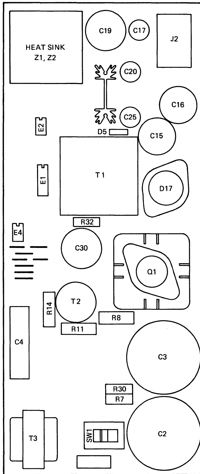
Figure 5-45 Power Supply Module, Component Locations
