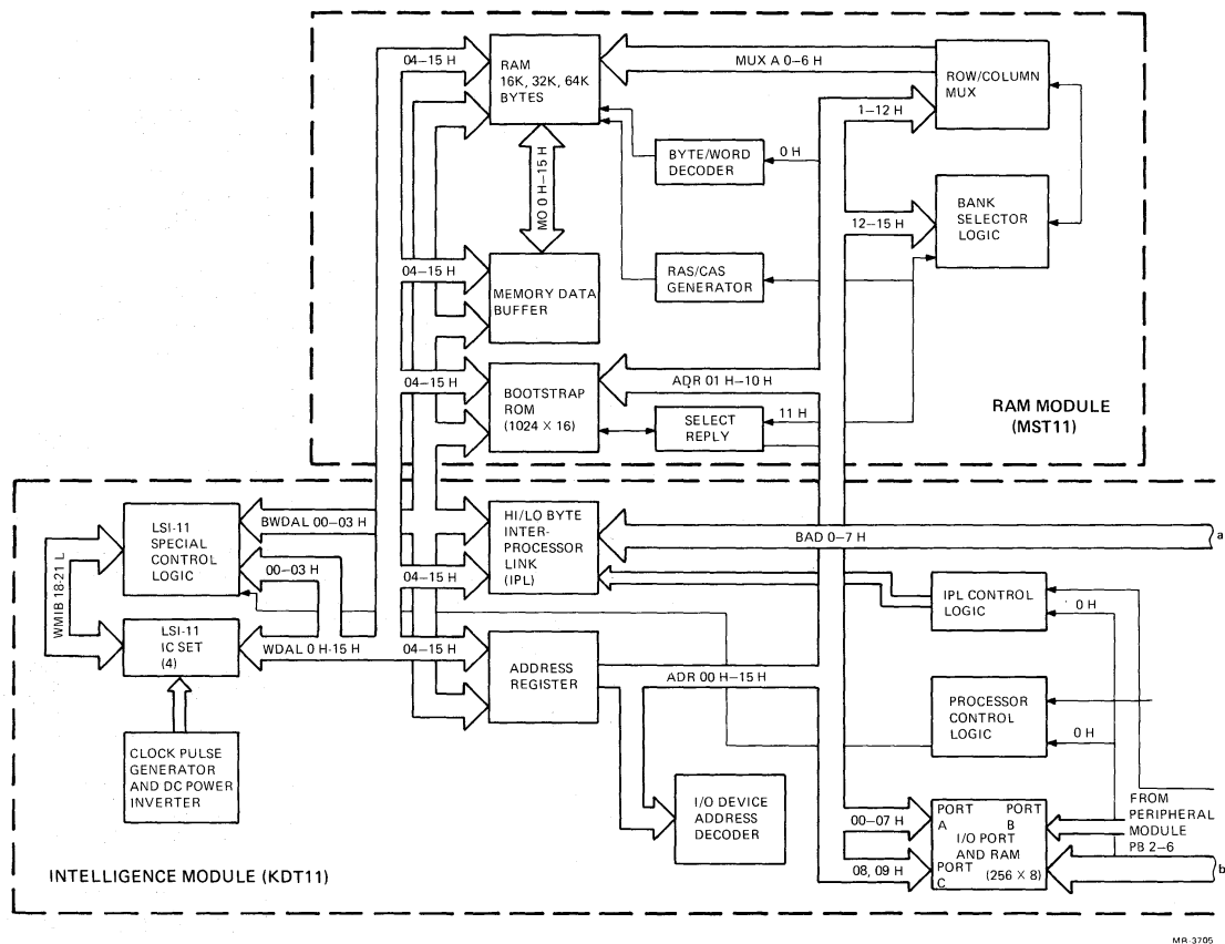
Figure 4-2 PDT-11/150 Bus Structure (Sheet 1 of 3)
