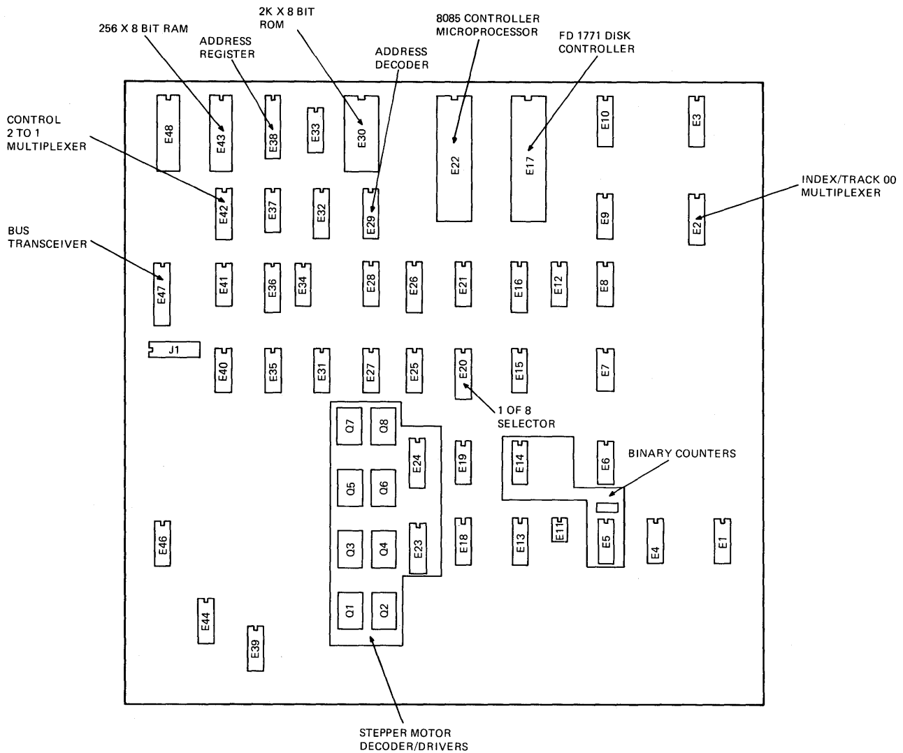
Figure 5-44 Disk Controller Module (Revision L), Functional Layout
