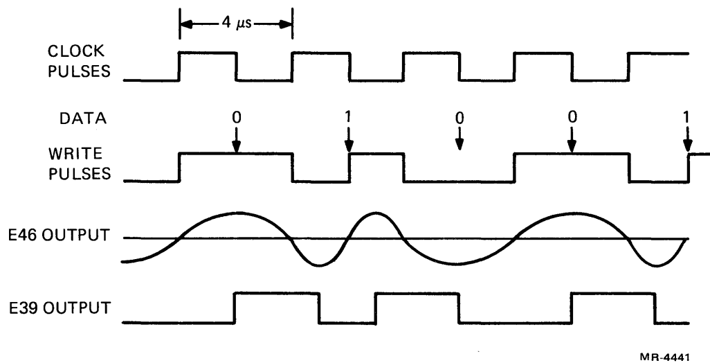
Figure 4-43 Read Amplifier and Differentiator Circuit (Revision K), Timing Diagram
