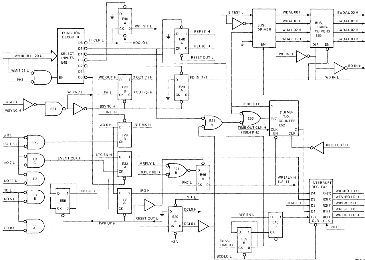
Figure 4-15 Function Control, Fast DIN and Interrupt Request Logic
