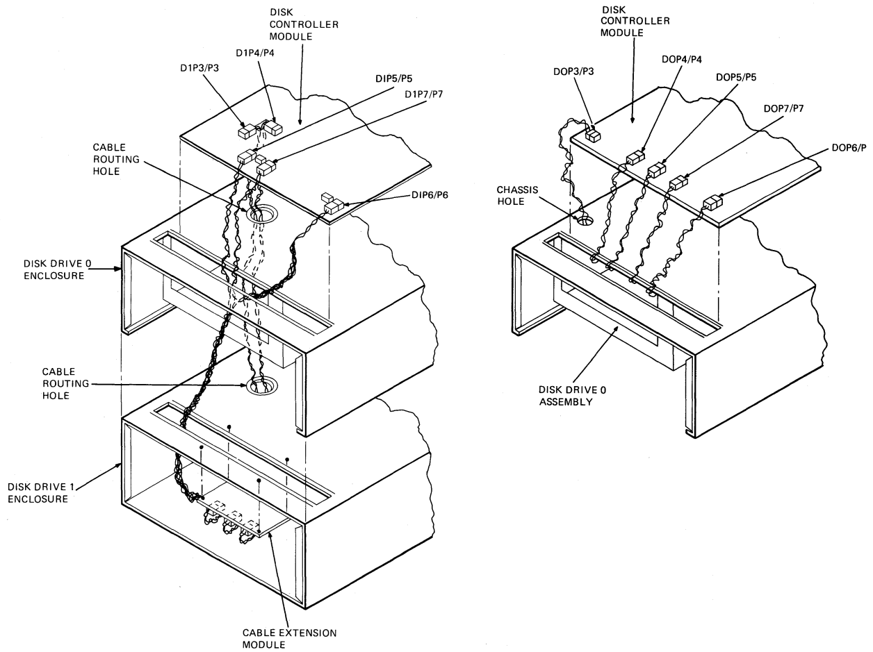
Figure 5-31 Disk Drive Cable Routing
