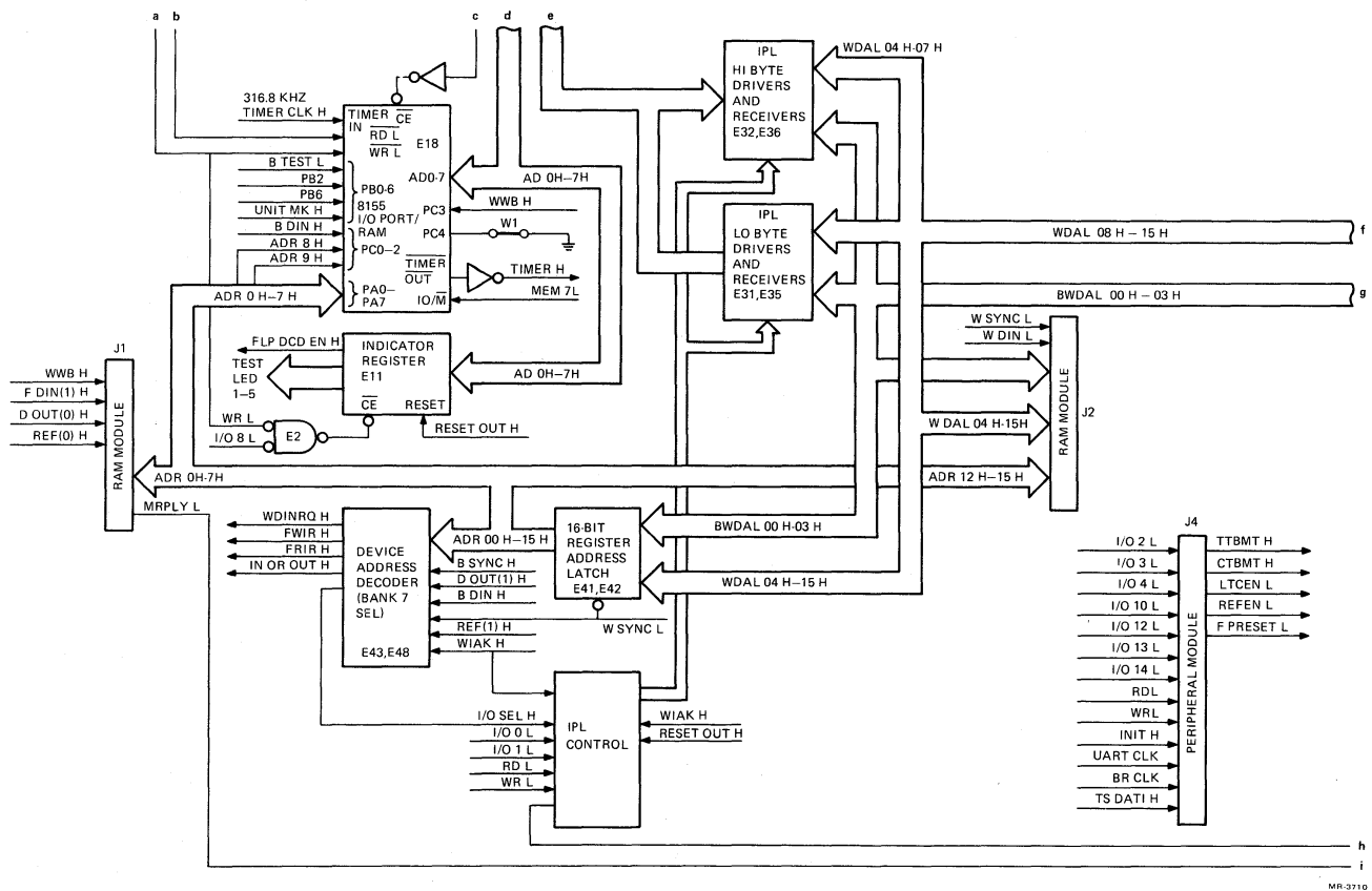
Figure 4-4 Intelligence Module, Simplified Function Diagram (Sheet 2 of 3)
