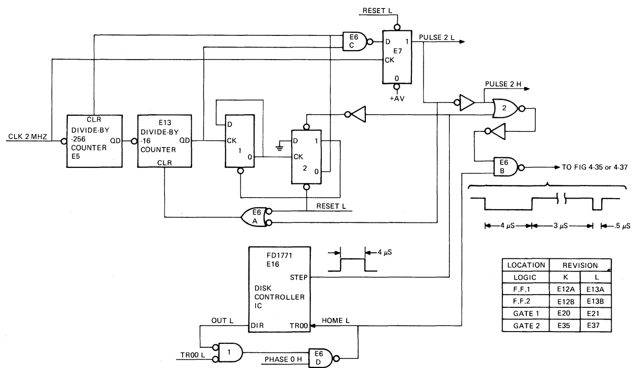
Figure 4-33 Step Generator Circuit, Simplified Diagram
