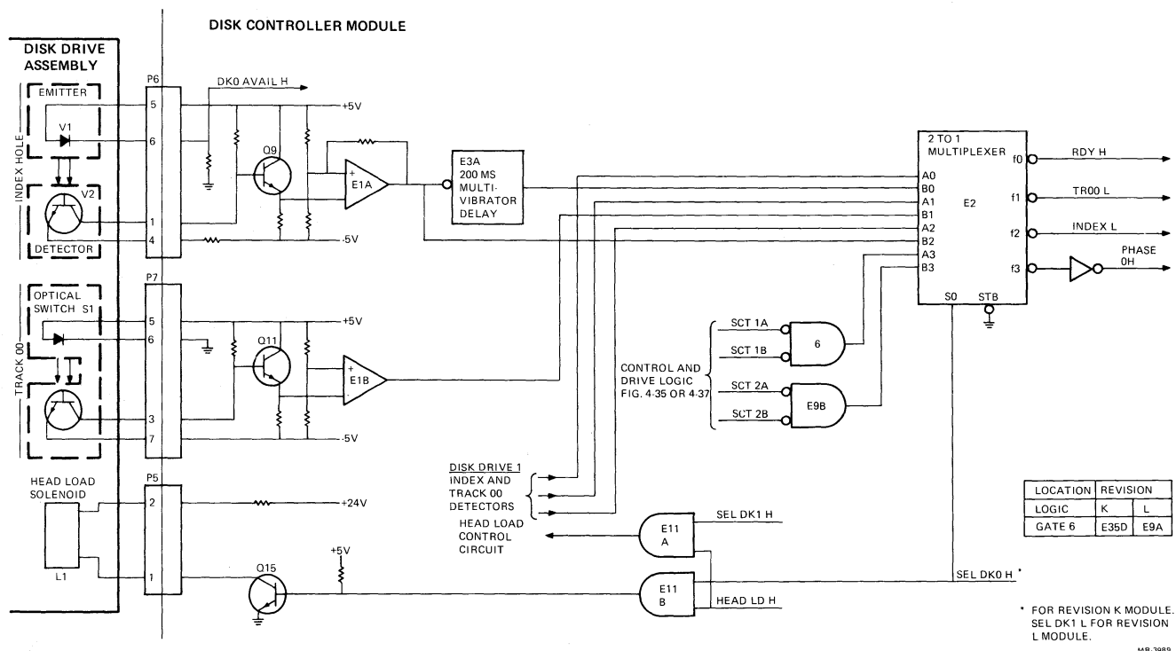
Figure 4-32 Head Load Control and Track and Index Hole Detection
