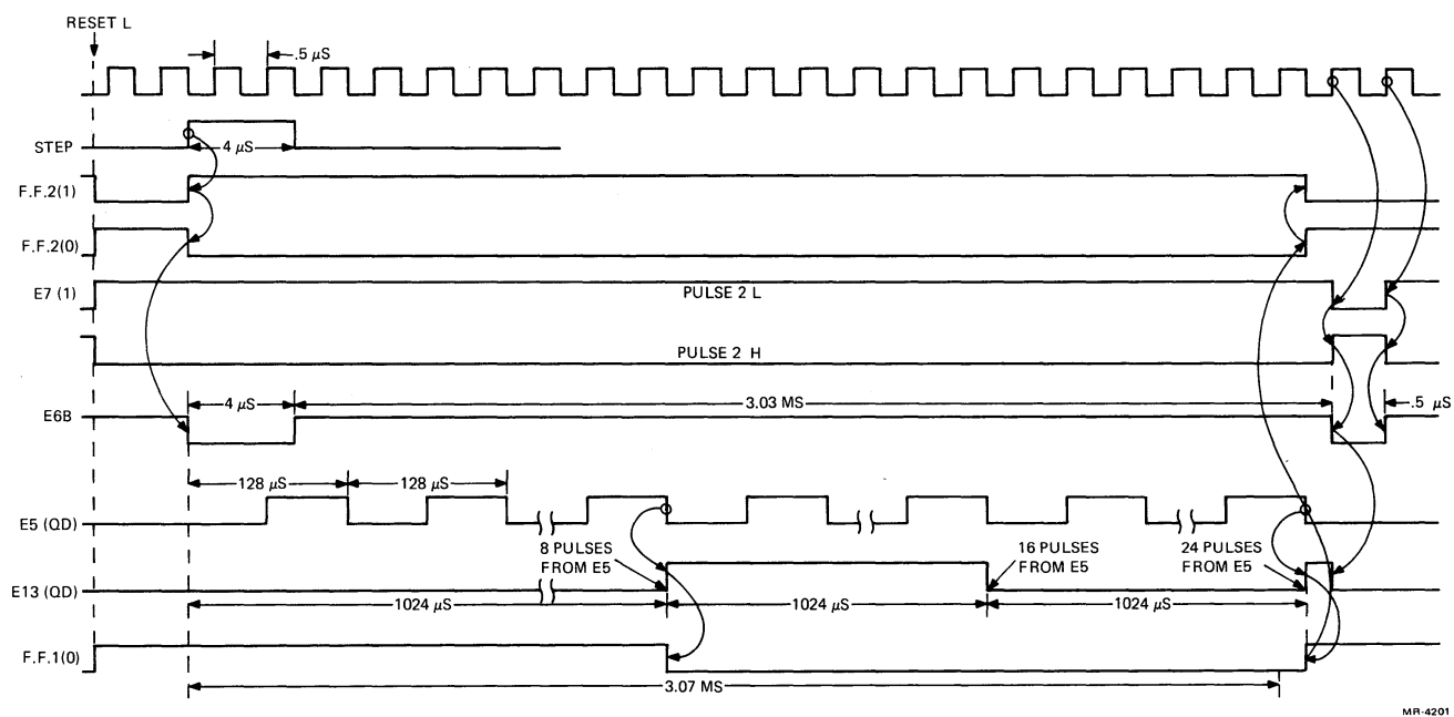
Figure 4-34 Step Generator Circuit, Timing Diagram
