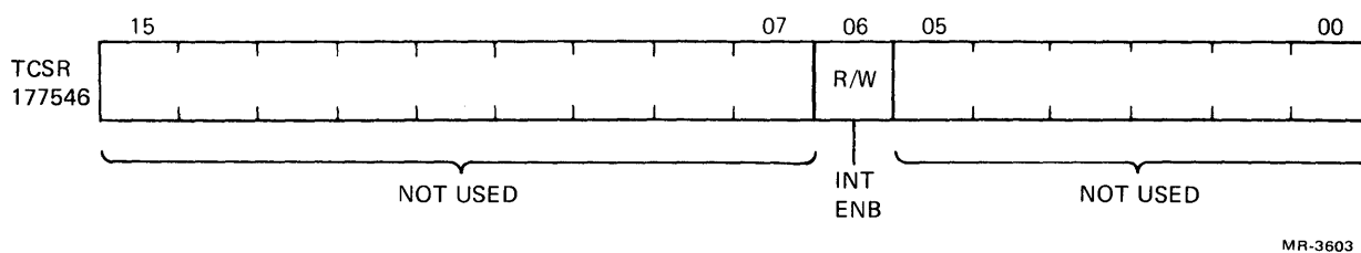
Figure 6-11 Line Time Clock (TCSR) Format
