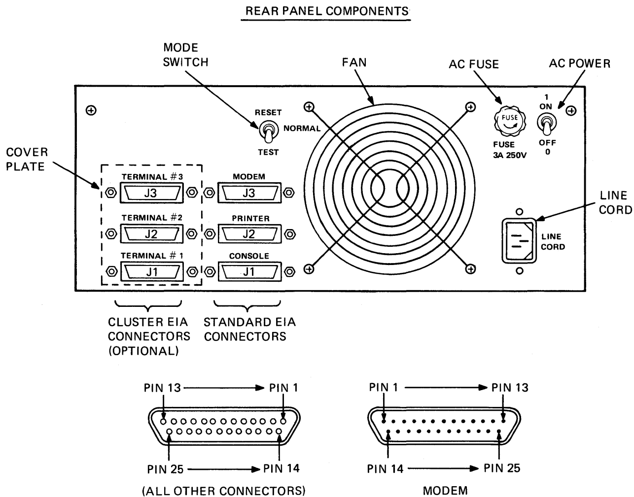
Figure 2-3 Rear Panel Assembly, Component and Connector Locations
