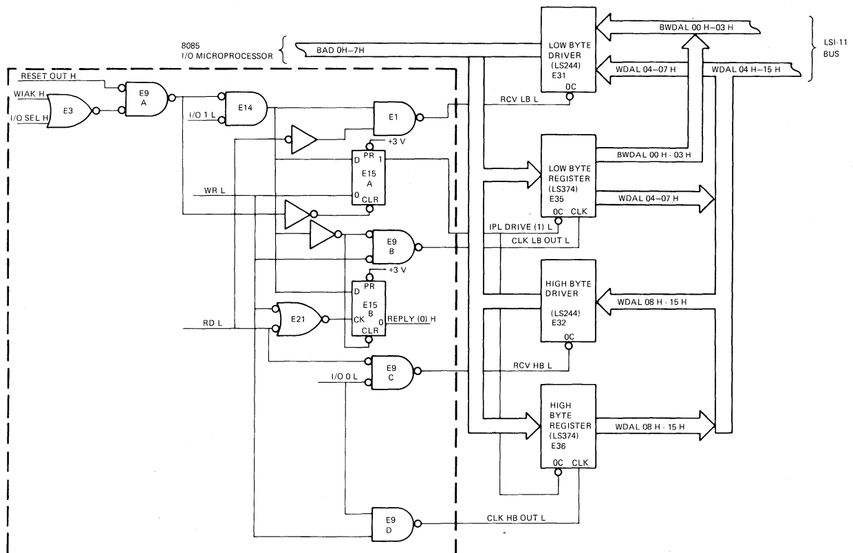
Figure 4-7 IPL and Control Logic, Simplified Diagram
