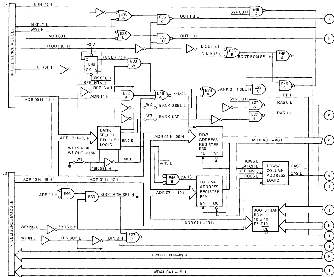
Figure 4-16 RAM Module, Simplified Function Diagram (Sheet 1 of 2)
