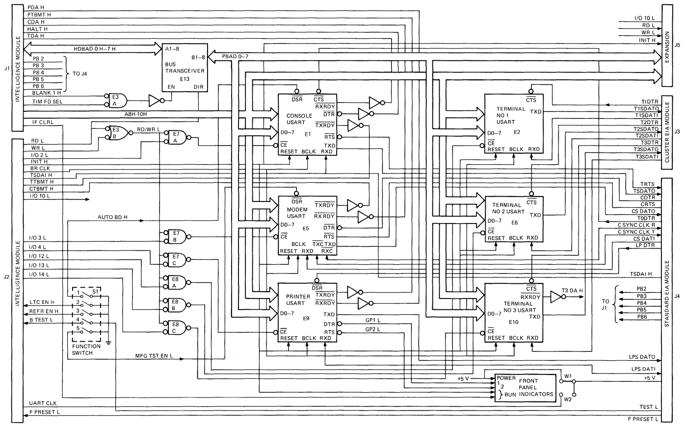
Figure 4-22 Peripheral Module, Simplified Function Diagram
