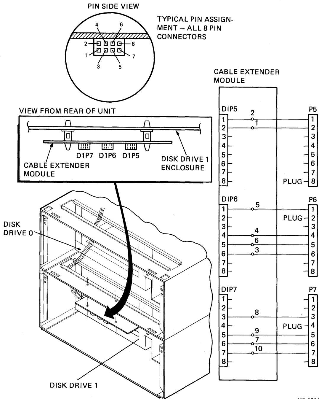
Figure 5-18 Cable Extender, Module Location and Connections
