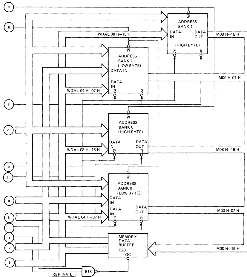
Figure 4-16 RAM Module, Simplified Function Diagram (Sheet 2 of 2)
