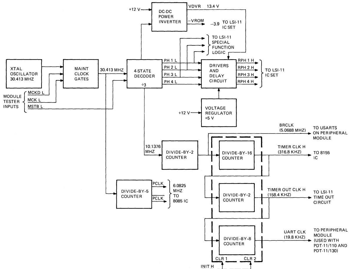
Figure 4-9 Clock Pulse Generator and Power Inverter, Simplified Block Diagram
