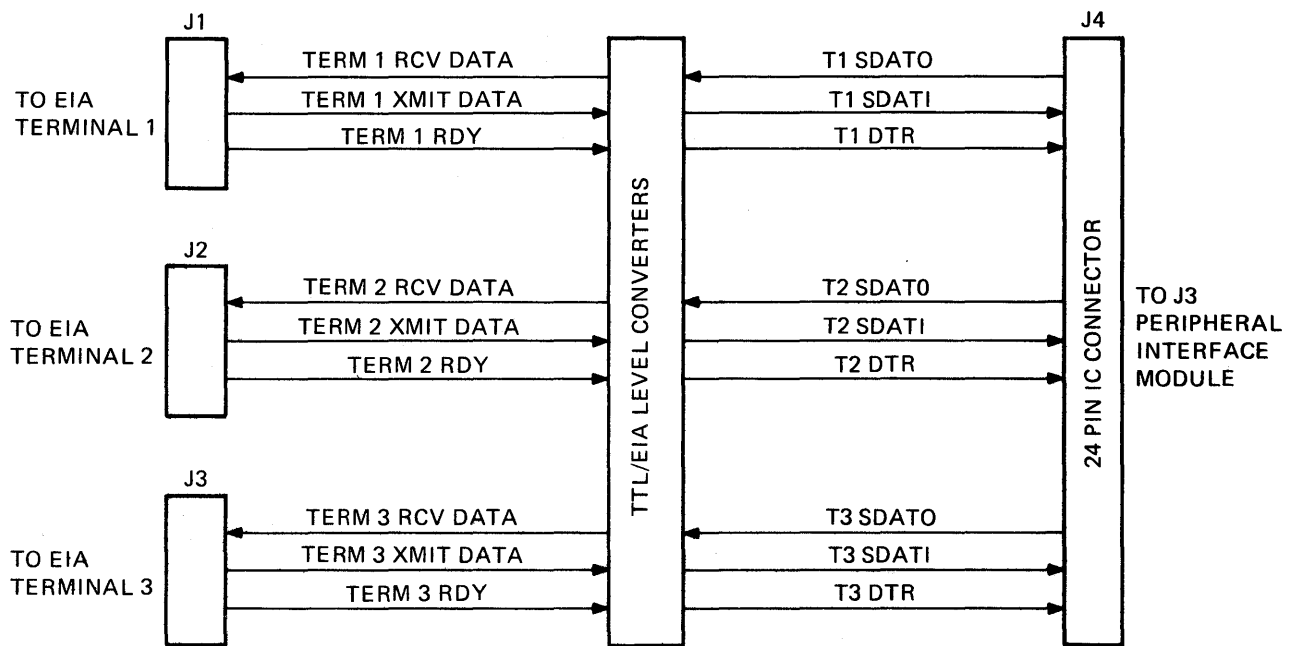
Figure 4-25 Cluster EIA Module, Simplified Diagram
