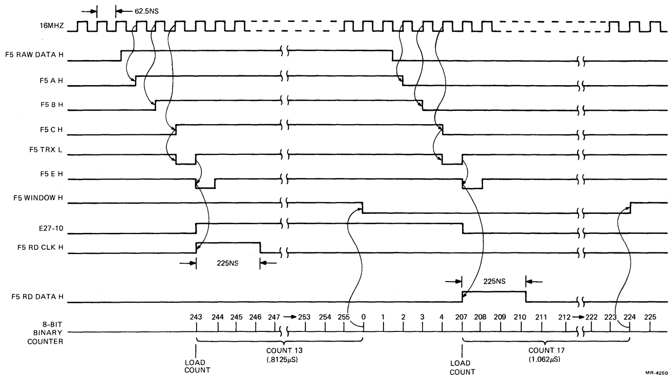
Figure 4-44 Data Separator Circuit (Revision L), Timing Diagram (Sheet 1 of 2)
