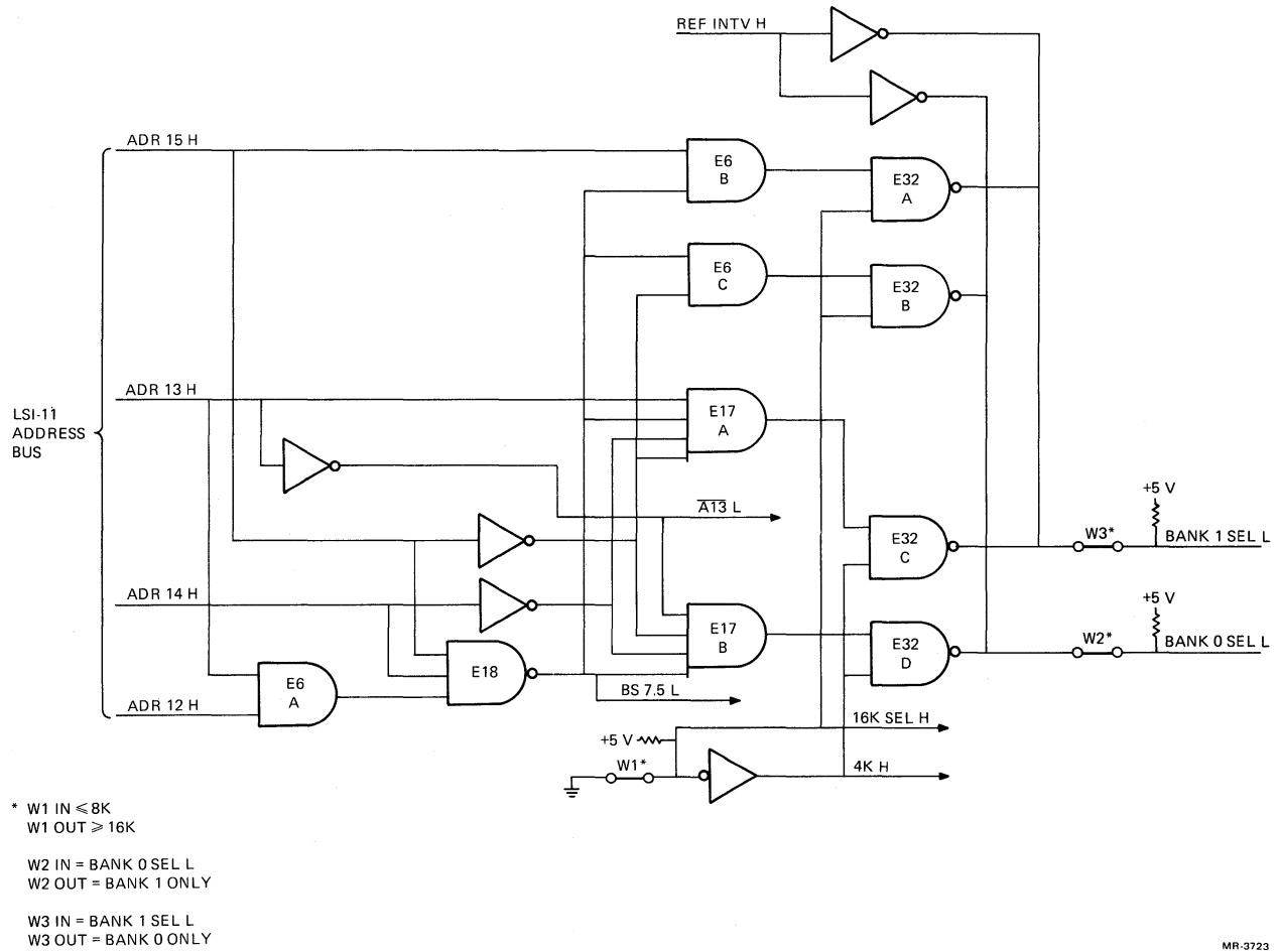
Figure 4-19 Bank Select Decoder Logic
