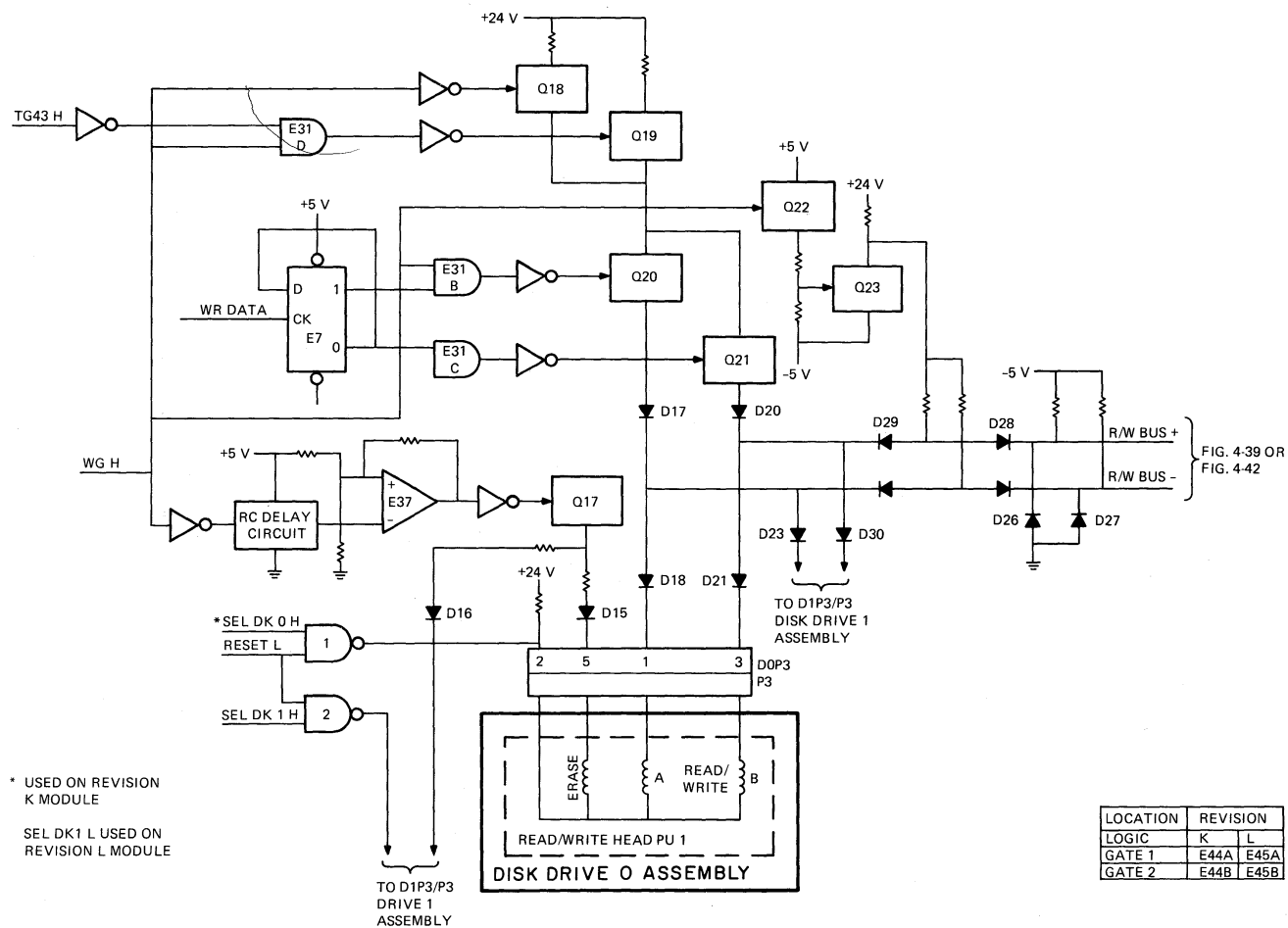
Figure 4-38 Read/Write Head and Control Circuits, Simplified Diagram
