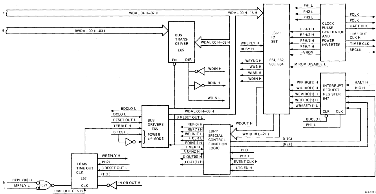
Figure 4-4 Intelligence Module, Simplified Signal Diagram (Sheet 3 of 3)
