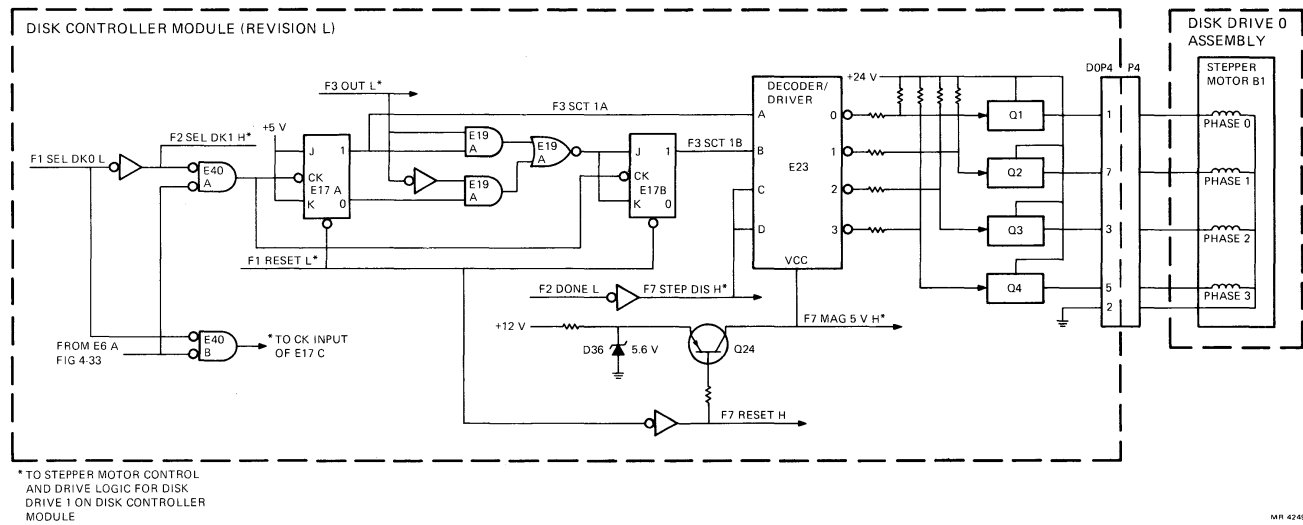
Figure 4-37 Stepper Motor Control and Drive Logic (Revision L), Simplified Diagram
