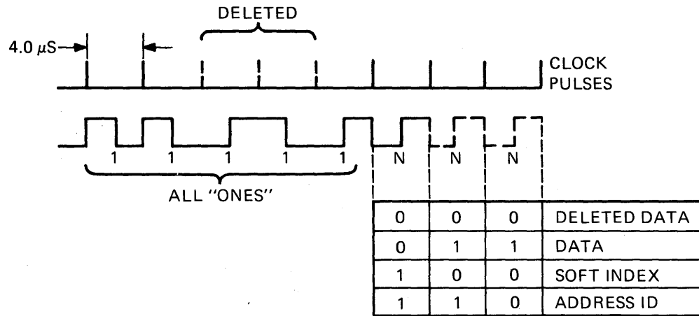
Figure 4-29 Double Frequency (FM) Address Mark Pattern
