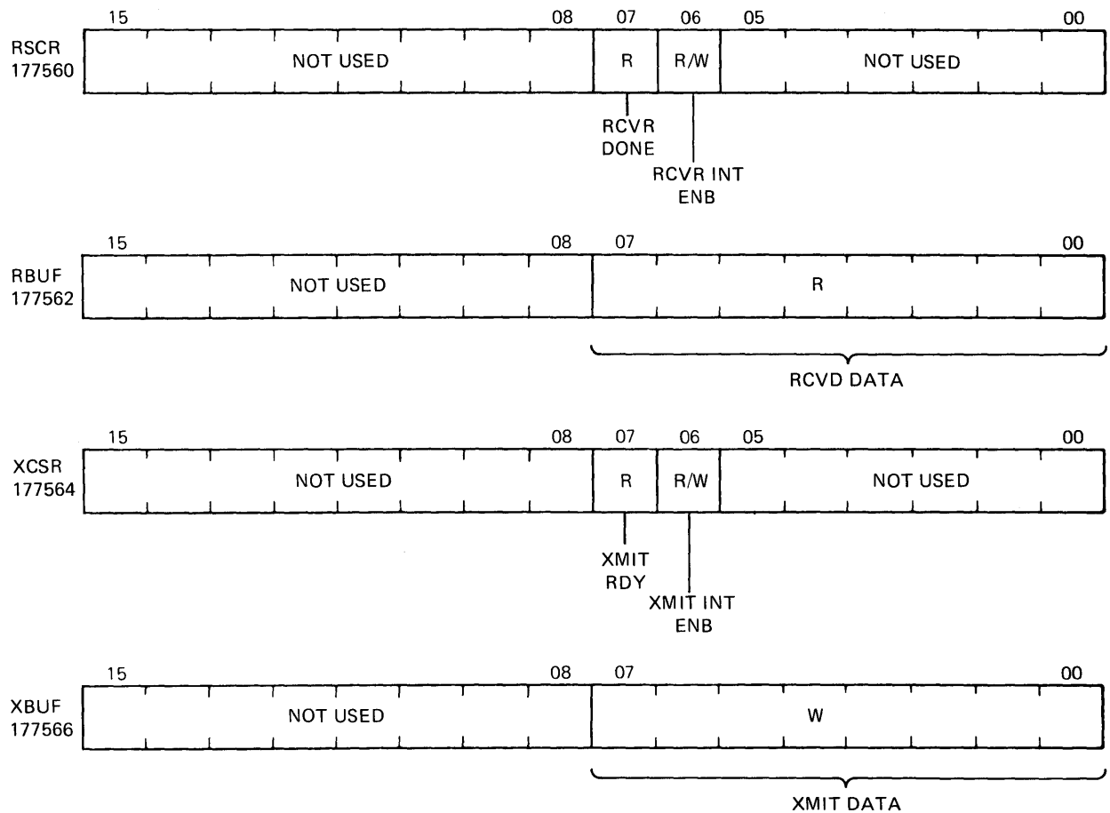
Figure 6-4 Console Terminal Interface Register Formats
