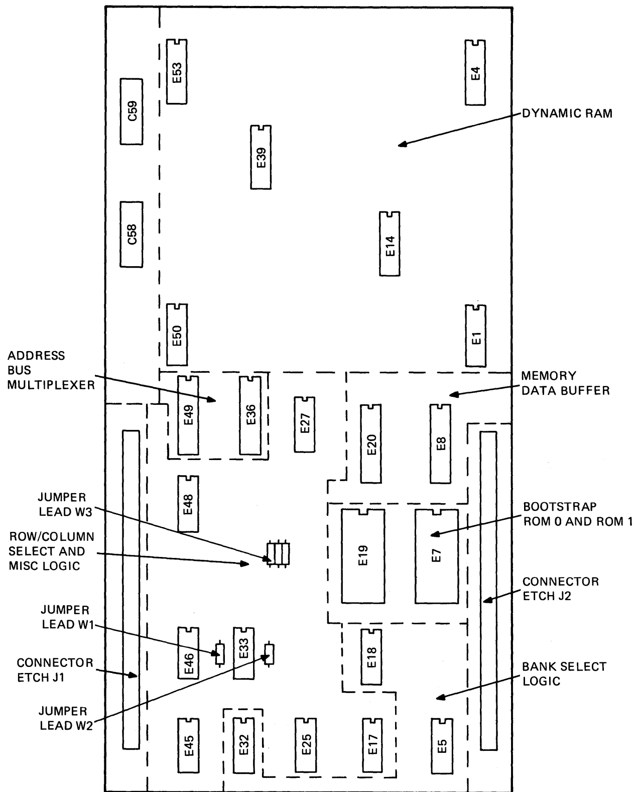
Figure 5-39 RAM Module, Functional Layout
