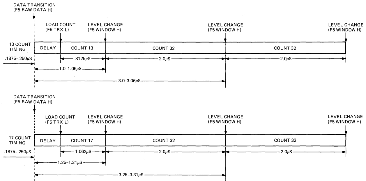
Figure 4-46 13- and 17-Count Intervals, Timing Diagrams
