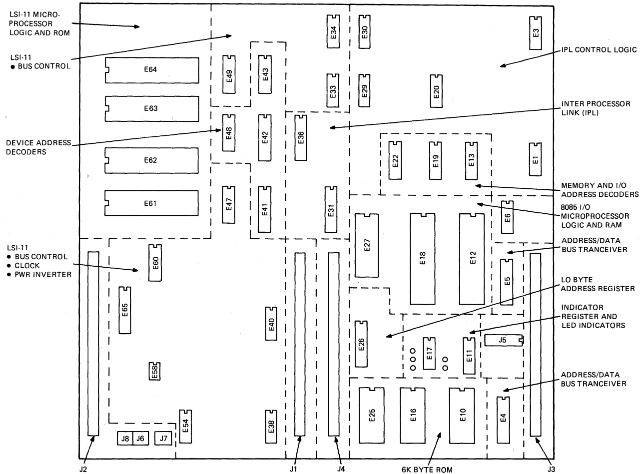
Figure 5-38 Intelligence Module, Functional Layout
