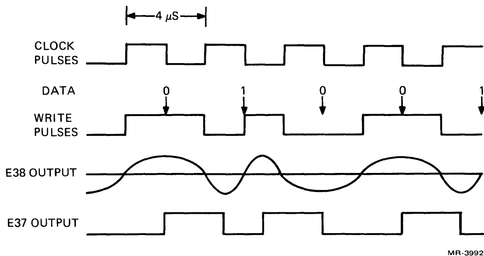
Figure 4-40 Read Amplifier and Differentiator Circuit (Revision K), Timing Diagram
