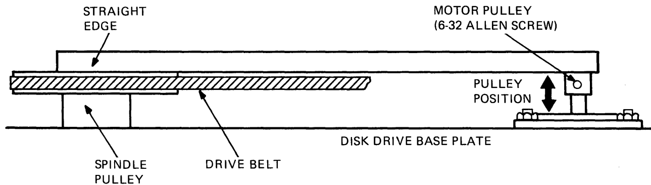
Figure 5-51 Pulley Alignment
