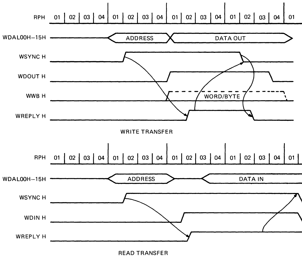
Figure 4-10 LSI-11 Microprocessor, I/O Transfer Timing (Sheet 1 of 2)
