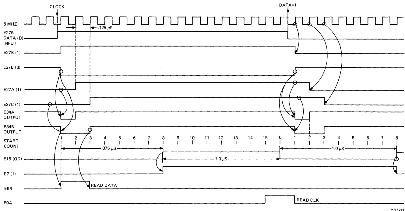
Figure 4-41 Data Separator Circuit (Revision K), Timing Diagram
