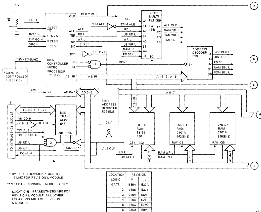
Figure 4-30 Disk Controller Module, Simplified Function Diagram (Sheet 1 of 2)
