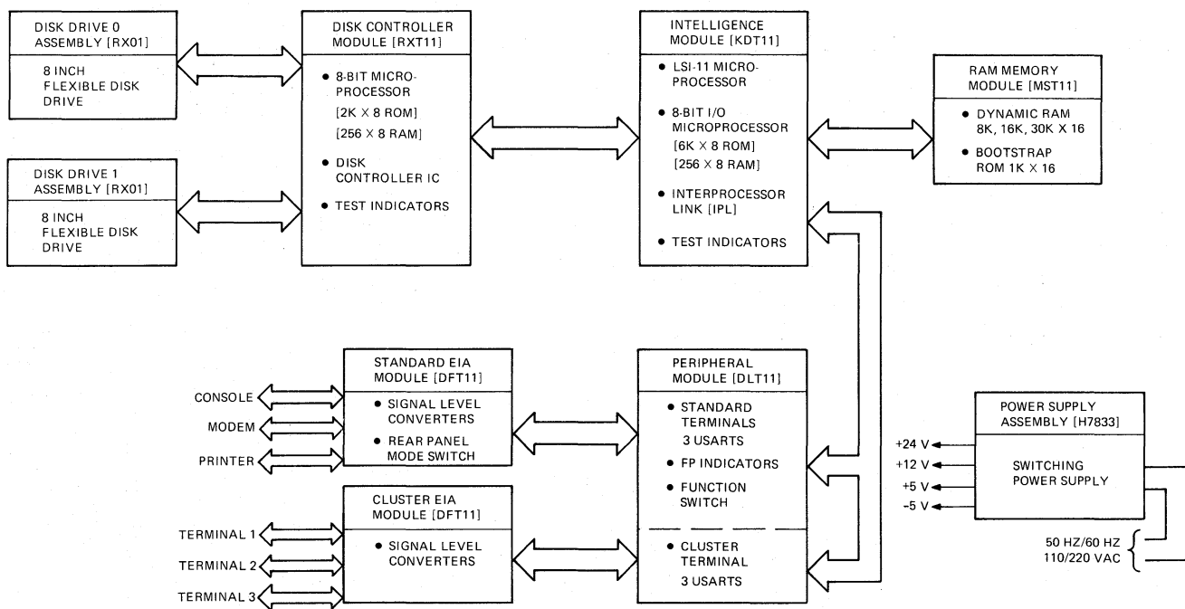
Figure 4-1 PDT-11/150, Simplified Block Diagram
